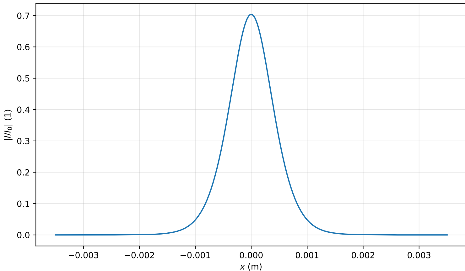
Intensity profile I(x, y = 0, z = 3.582m)/I_0 , P_{in}=0.7P_{cr} , artificial time
